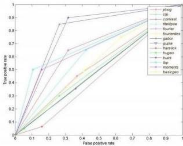
Fig. 4. The ROC curve: Crocodile vs crocodile head
