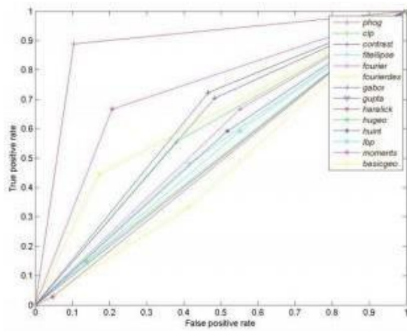
Fig. 3. The ROC curve: Crab vs crayfish
