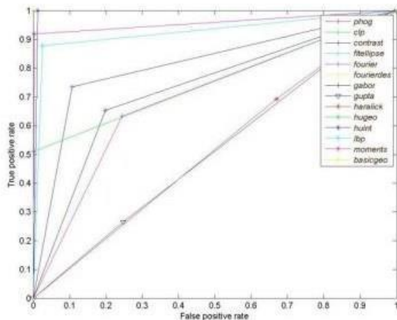
Fig. 1. The ROC curve: Airplanes vs car side
