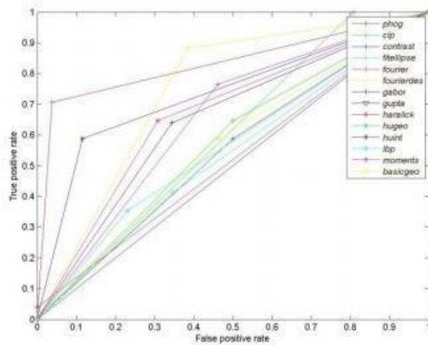
Fig. 5. The ROC: Flamingo vs flamingo head
